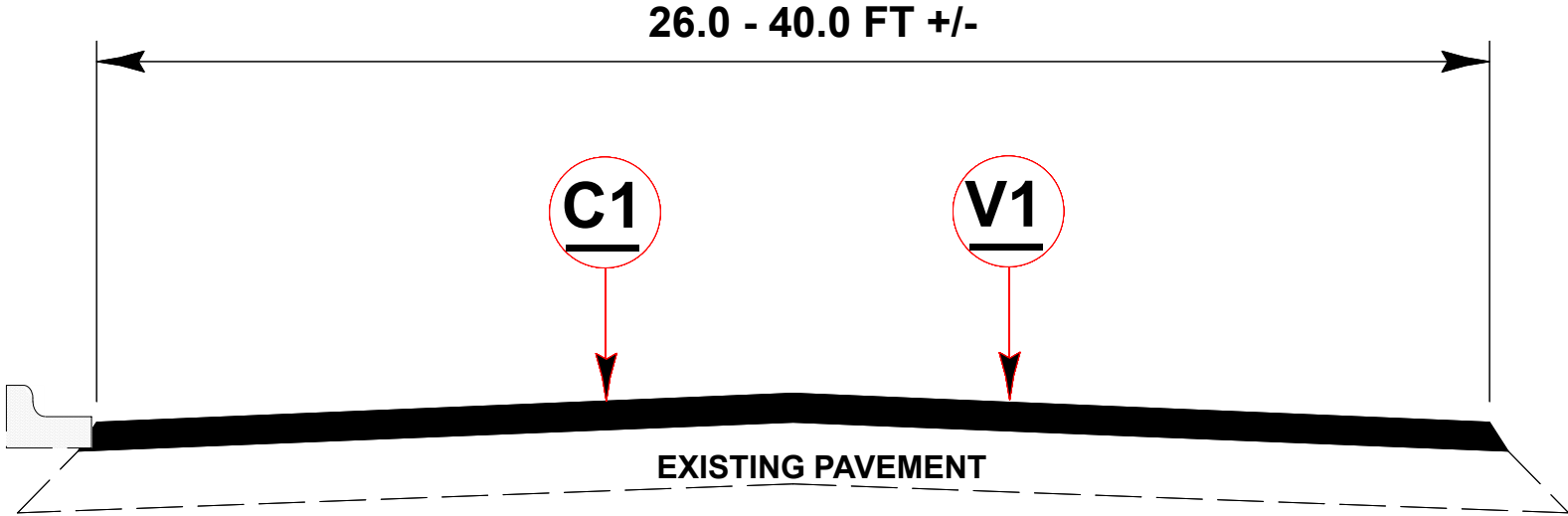
TYPICAL SECTION # 3 MAP(S) # 3
